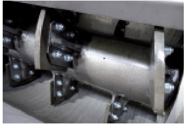
Fig. 8: Replaceable wear paddle - No balancing of shaft required - Interchangeable screens without welding - Stainless steel and galvanized components provide optimized corrosion protection
