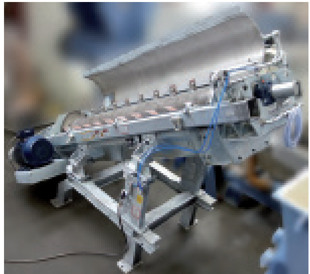
Fig. 9: Pneumatic opening device for maintenance work reduces downtime.
